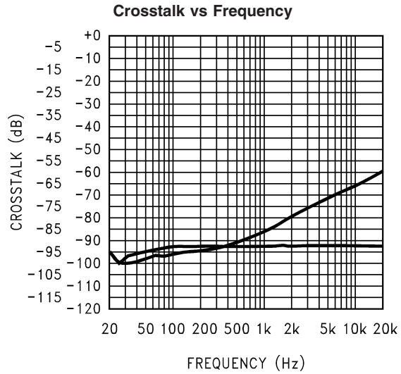
20079737 V DD = 3V; LHP, RHP; P O = 10mW; R L = 32Ω; Mode 9; 0db Gain; 3D off Top-Left to Right; Bot- Right to Left
