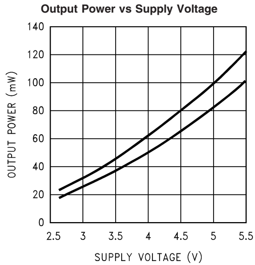
LHP, RHP; R_L = 32\Omega ; Top-10% THD+N; Bot-1% THD+N
