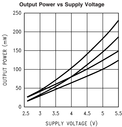
EP; R_L = 32\Omega ; Top-10% THD+N; CD4 = 1; Topmid-1% THD+N, CD4 = 1 Botmid-10% THD+N; CD4 = 0; Bot-1% THD+N, CD4 = 0
